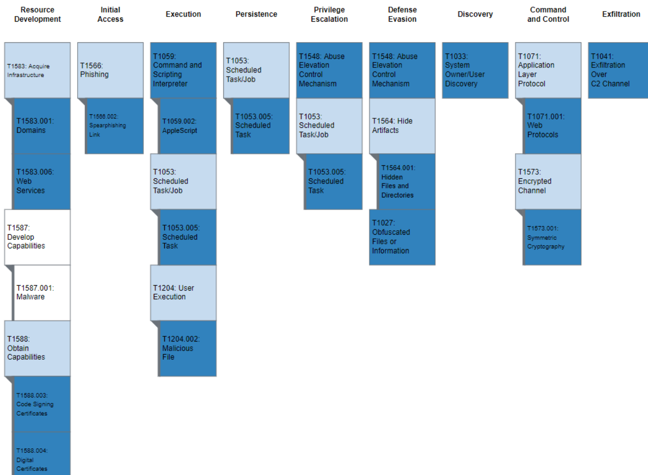
Figure 2: MITRE ATT&CK enterprise techniques used by AppleJeuS
